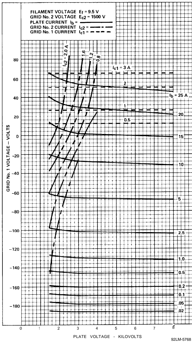
Figure 5 - Typical Constant Current Characteristics
